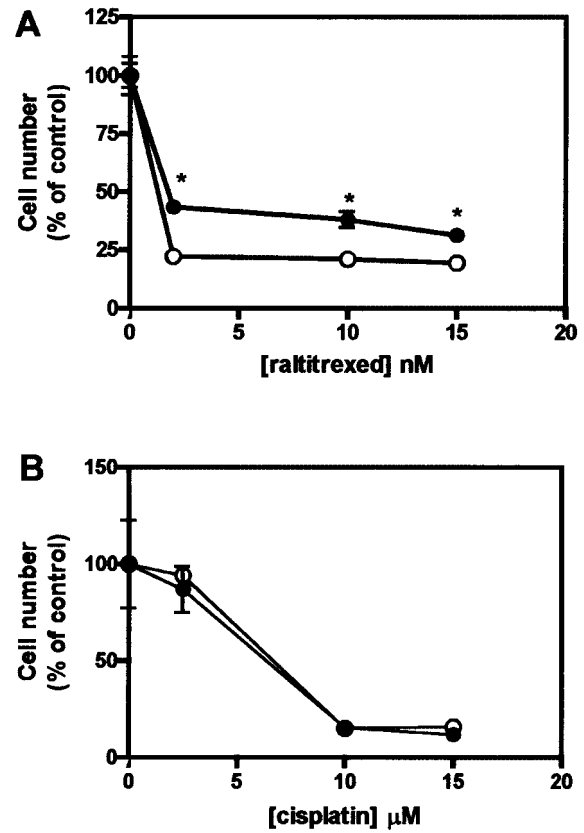
Figure 9. Effect of a TS expression vector on HeLa cell sensitivity to raltitrexed and cisplatin. Cells were transfected with control GFP plasmid (2.0 μg, open symbols) or TS-14 plasmid (2.0 μg, solid symbols) and proliferation assessed in the presence of a range of concentrations of raltitrexed (A) or cisplatin (B) as described in Materials and Methods. Proliferation of cells transfected with TS-14 is shown relative to proliferation of cells transfected with GFP. Data are presented as mean ± SD (n = 3). *Different from cells treated with GFP (p < 0.05, Student's t-test).
